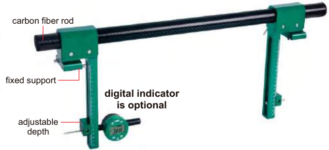
measure inside diameter, minimum diameter is 220mm
