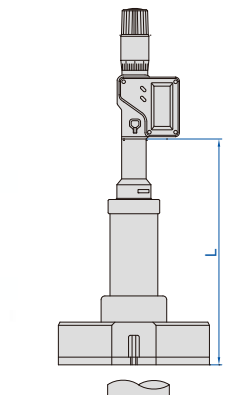
type D 50-300mm, carbide measuring points three points
